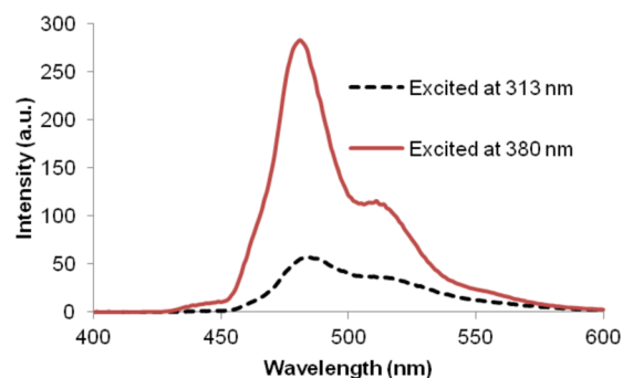
Figure 7. Photoemission spectrum of trans -Pt(PEt 3 ) 2 (peryl)(Cl) 3 2 (R = peryl) in CH 2 Cl 2 . Solid red line for 380 nm excitation and dashed black line for 313 nm excitation.
