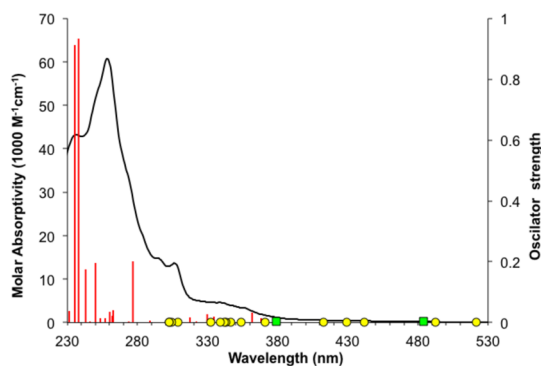
Figure 12. UV-vis absorption spectrum of trans -Pt(PEt 3 ) 2 (Cl) 3 (phen) 2 (R = phen) in dichloromethane (black line) and TDDFT (CAM-B3LYP, pcm) vertical transitions for trans -Pt(PMe 3 ) 2 (Cl) 3 (phen) 2' (R = phen) (red vertical lines, height corresponds to the oscillator strength). Yellow circles mark calculated triplet transitions (>300 nm), and green squares mark calculated dark (oscillator strength <0.01) singlet transitions (>370 nm).
