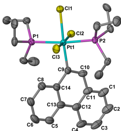
Figure 1. Solid-state structure of one of two independent molecules of 2 ( R = \text{phen} , 50% probability ellipsoids, hydrogen atoms omitted). The second molecule shows a rotational disorder in the phenanthryl ring system (Supporting Information).
