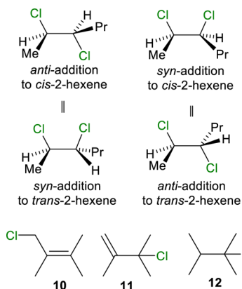
Figure 4. TME and cis - and trans -2-hexene products from the photolysis of 2 . Only one enantiomer shown for chiral 2-hexene products.
