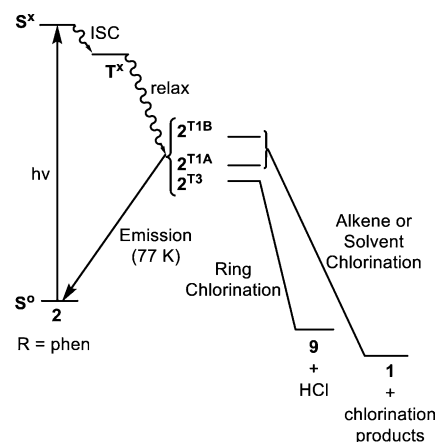
Scheme 4. Proposed Jablonski-type Diagram for 2 (R = phen) a
