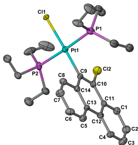
Figure 3. Solid-state structure of 9 ( R_{Cl} = Cl\text{-phen} ) (30% probability ellipsoids, hydrogen atoms omitted). A second orientation of one ethyl group on each phosphine ligand is not shown.
